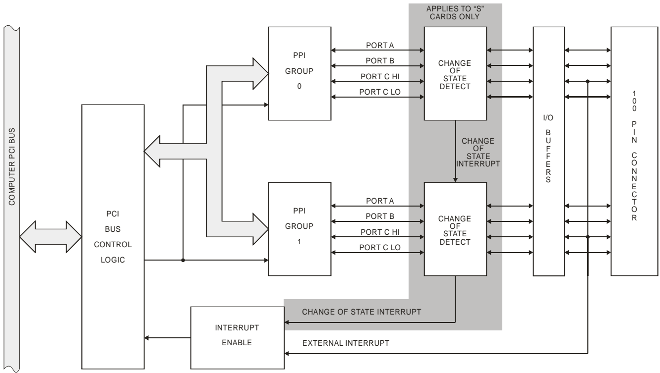
Figure 1-1: Block Diagram
